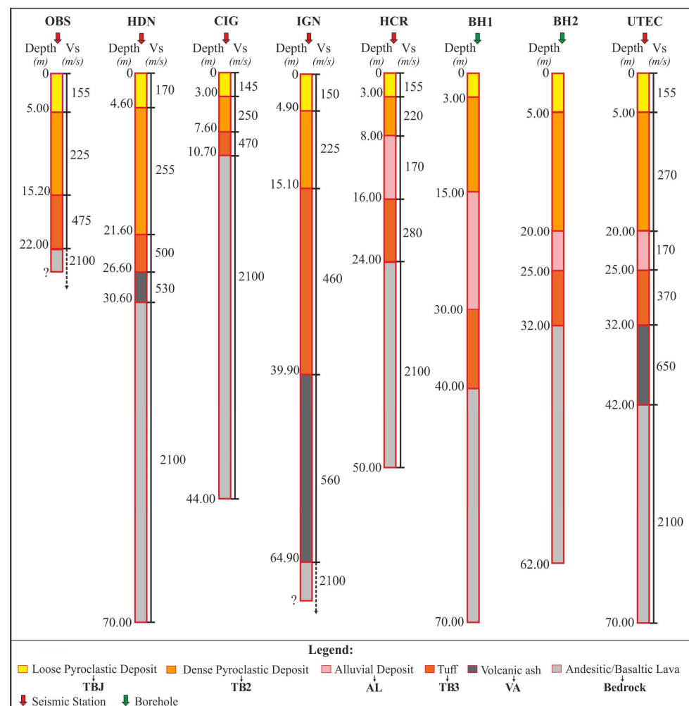
Figure 4. Seismic-litho-technical sections of eight sites located within the MASS area are used for the reconstruction of both subsurface models (AA', BB').
