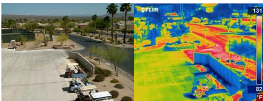
Figure 2. The infrared image demonstrates that the light colored concrete remains cooler than the darker colored asphalt road.
