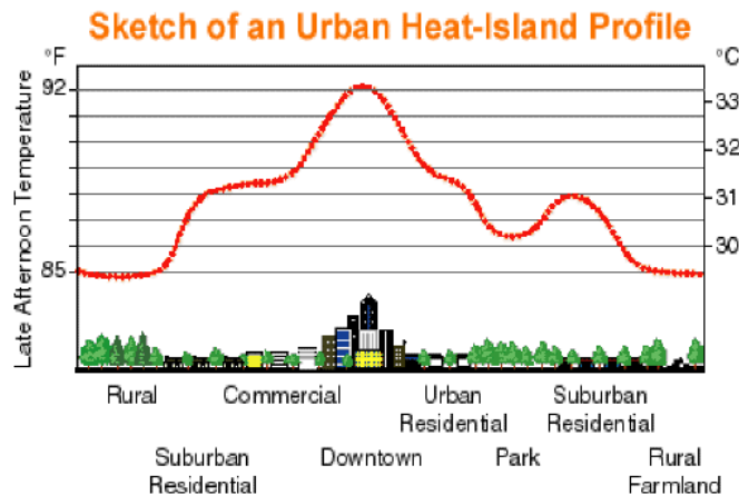
Figure 1. Urban Heat Island Profile [5].
