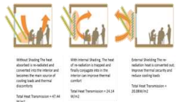
Figure 7. Fenestration System Thermal Performance (Al-Tamimi, Fadzil, & Harun, 2011)
